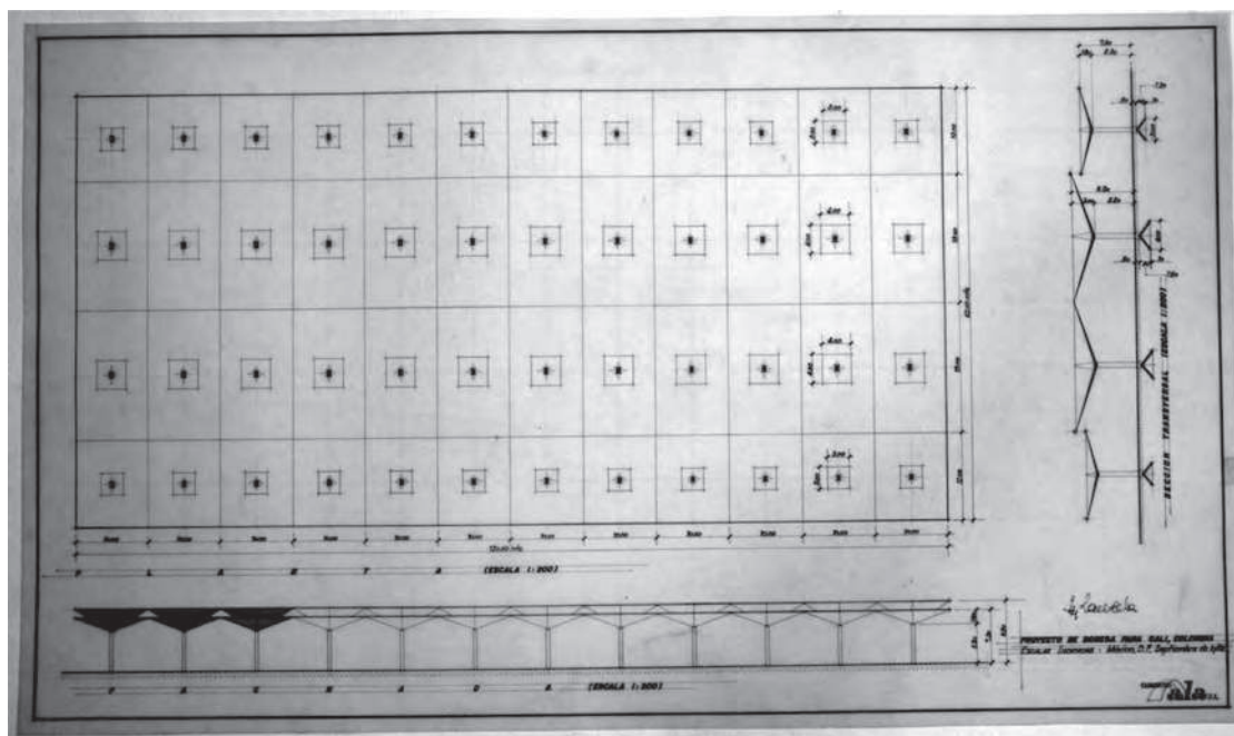
Figura 3. Almacén en Cali de Cubiertas Ala Colombia. Félix Candela architectural records and papers, 1950-1984, Avery Architectural & Fine Arts Library, Columbia University.
