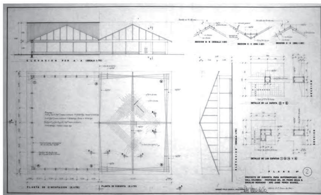
Figura 4. Supermercado Belmonte en Cali de Cubiertas Ala Colombia. Félix Candela architectural records and papers, 1950-1984, Avery Architectural & Fine Arts Library, Columbia University.
